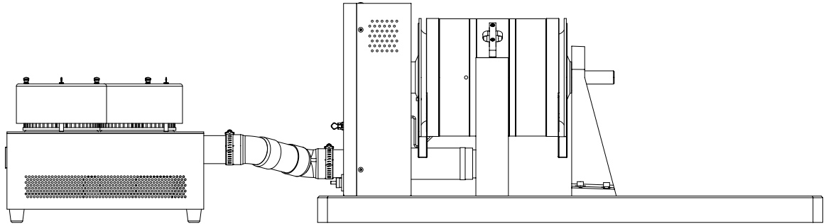
Figure 3–9 Dynamometer with Blower Connection
