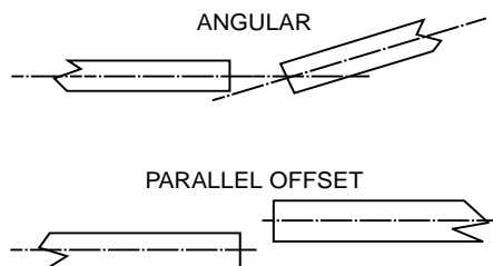
Figure 4–3 Examples of Possible Shaft Misalignment
