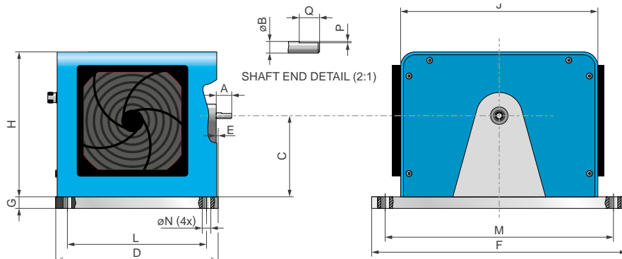
Fig. 4: HD-400 Dynamometer with short base plate
