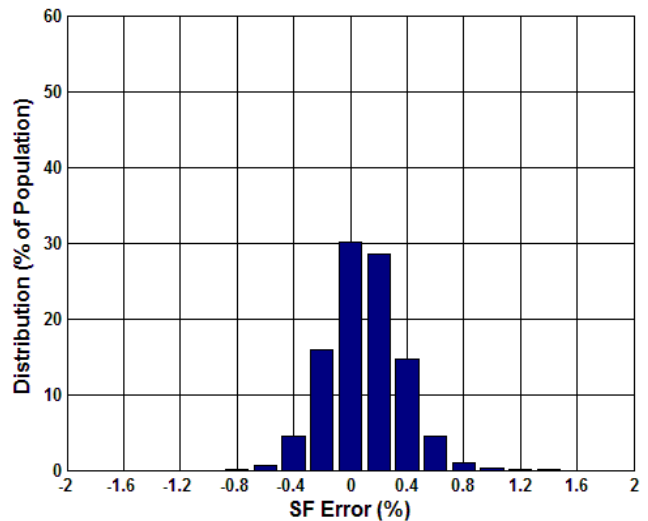
Figure 5.39 Digital SF Error (%) over Temperature
