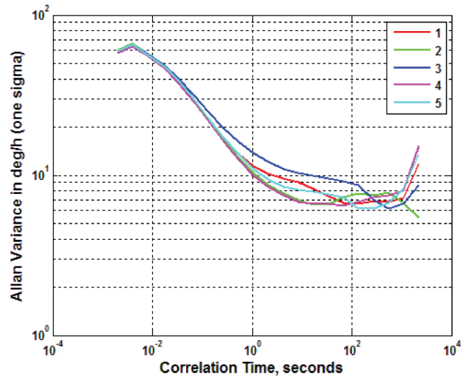
Figure 5.52 Allan Variance of CRM100s 75°/s 25Hz
