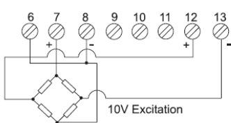
Transducer Supply
