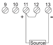
Current ( \pm 20\text{mA} )
