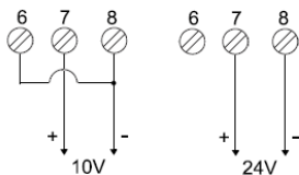
Transducer Supply
